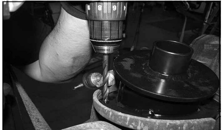
FIGURE 14 - STEP 24
